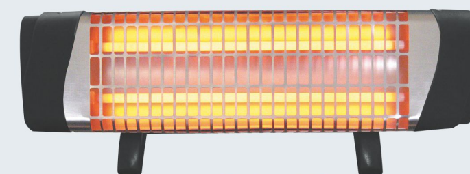
QH-1200M Power:1200W Meas(mm):615x160x135 Qty/40'HQ:4900pcs
