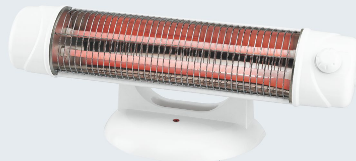
QH-1200A Power:1200W Meas(mm):590x185x235 Qty/40'HQ:2470pcs
